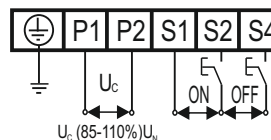
Wiring Drawing
