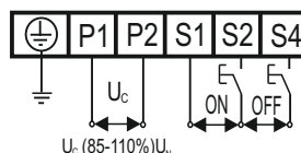
Wiring Drawing
