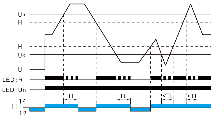
Functions Diagram
