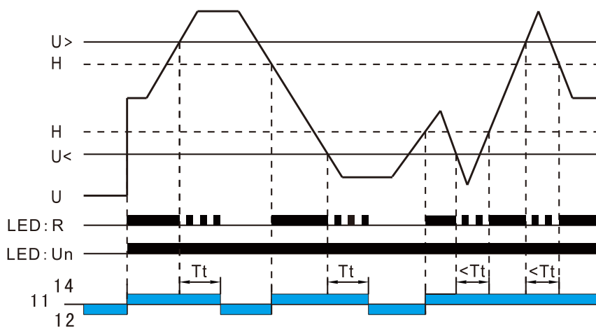
Functions Diagram
